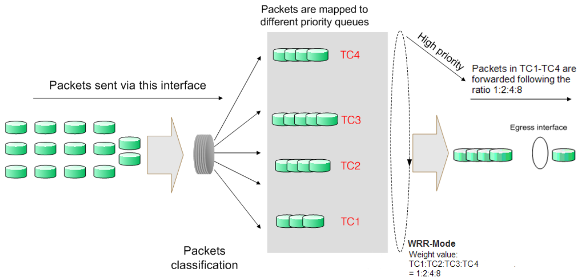
Figure 8-1 QoS function
