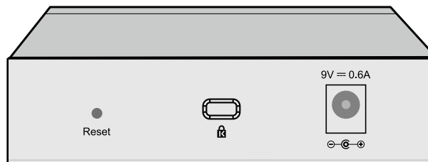
Figure 2-7 Rear Panel of TL-SG105E
